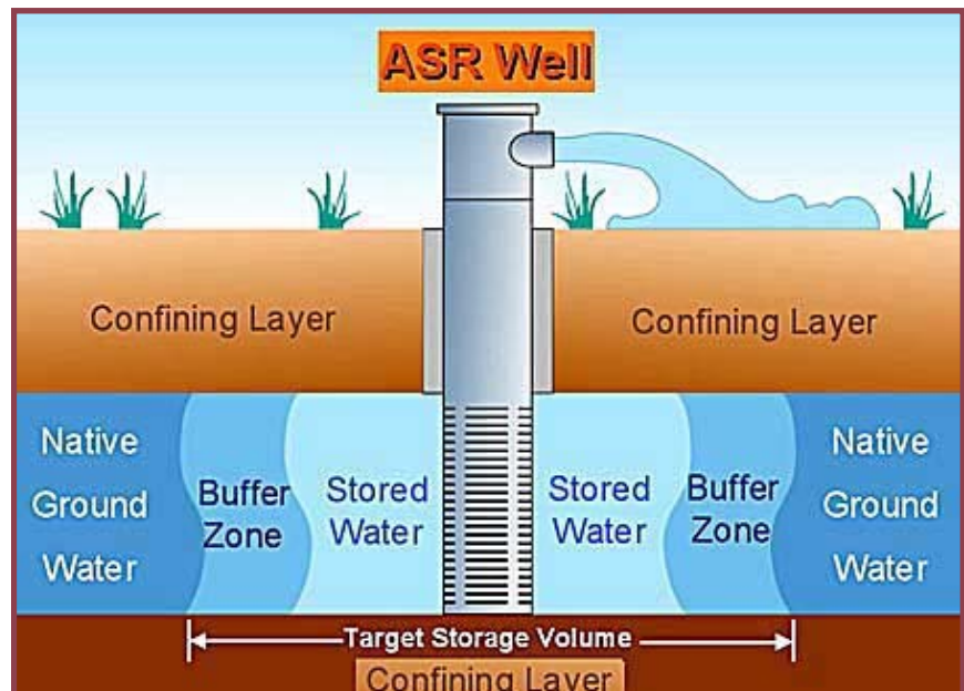
Figure 23, ASR Well
