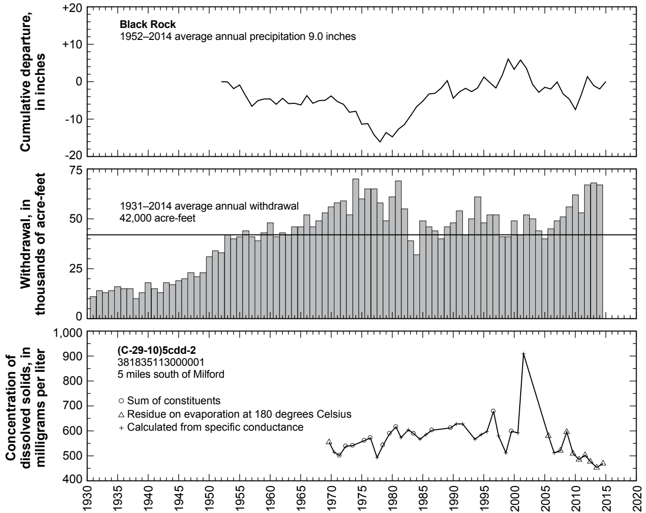
Figure 42. Relation of water level in selected wells in the Milford area to cumulative departure from average annual precipitation at Black Rock, to annual withdrawal from wells, and to concentration of dissolved solids in water from well (C-29-10)5cdd-2.— Continued
